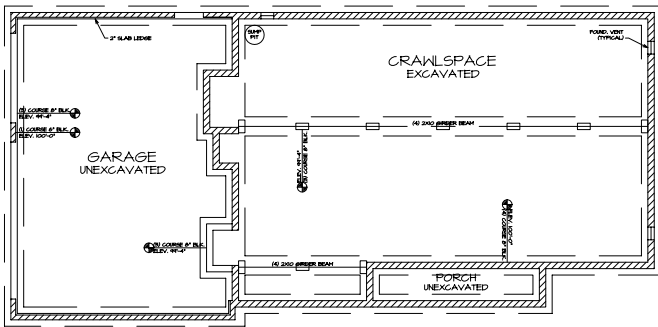
1 FOUNDATION PLAN A-3 SCALE: 1/4"=1'-0"
