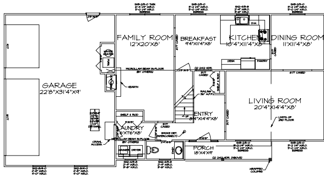
1 FIRST FLOOR PLAN A-4 SCALE: 1/4"=1'-0"
