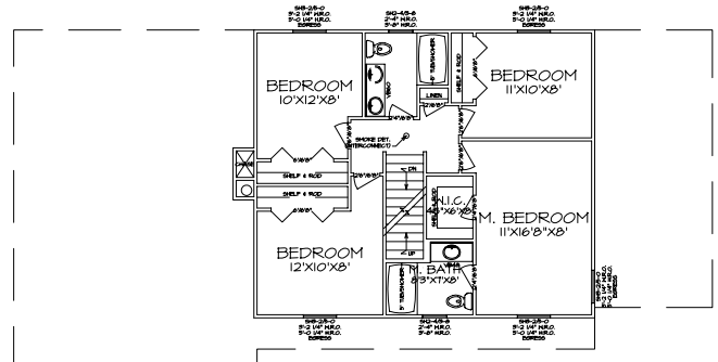
1 SECOND FLOOR PLAN A-5 SCALE: 1/4"=1'-0"
